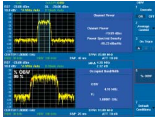
Simultaneous measurement of Channel Power and OBW
